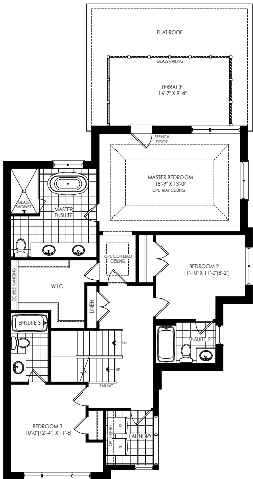
SECOND FLOOR PLAN ELEV. 'A'
