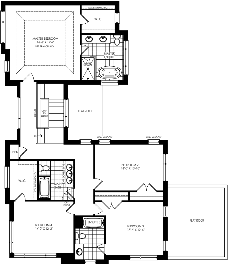
THIRD FLOOR PLAN ELEV. 'A'
