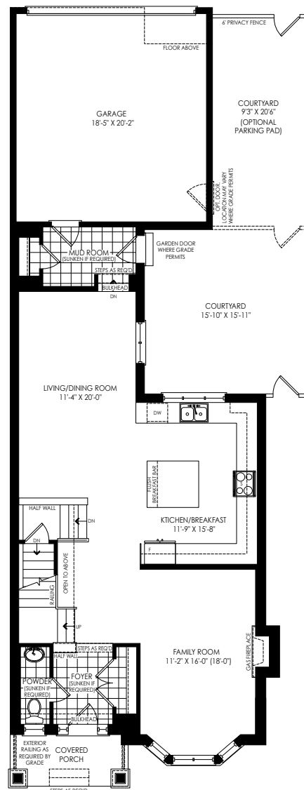
GROUND FLOOR PLAN ELEV. 'D'
