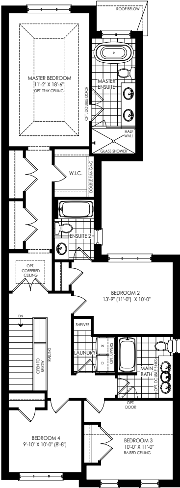
THIRD FLOOR PLAN ELEV. 'B'
