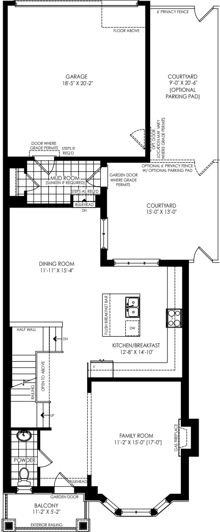
SECOND FLOOR PLAN ELEV. 'D'
