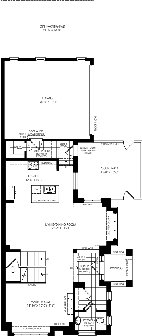
GROUND FLOOR PLAN ELEV. 'E'
