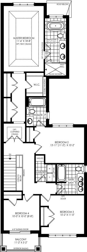
THIRD FLOOR PLAN ELEV. 'D'
