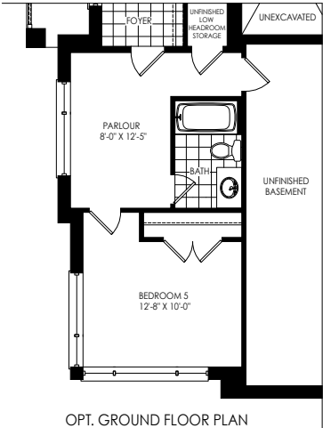
OPT. GROUND FLOOR PLAN W/ 5 BEDROOMS ELEV. 'A'
