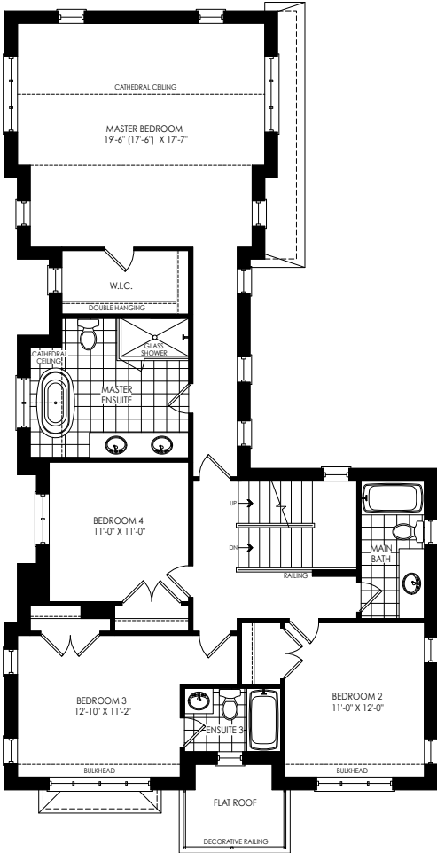
SECOND FLOOR PLAN ELEV. 'E'
