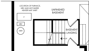
PARTIAL OPT. BASEMENT PLAN W/ FINISHED LANDING ELEV. 'E', 'B', 'D' & 'A'
