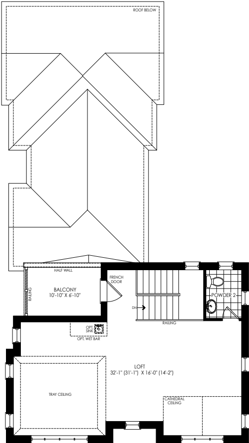
LOFT PLAN ELEV. 'E'
