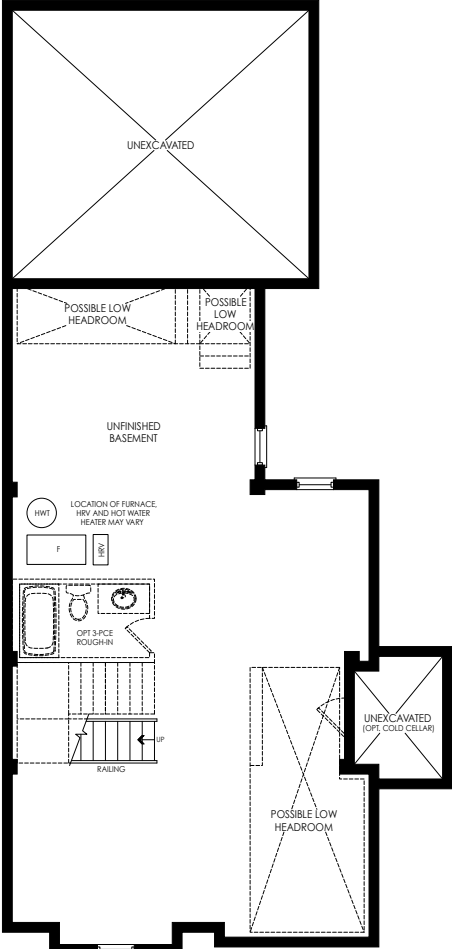
BASEMENT PLAN ELEV. 'B'
