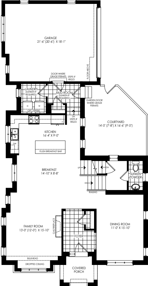
GROUND FLOOR ELEV. 'E'
