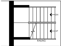
PARTIAL GROUND FLOOR PLAN FOR OPT. FINISHED BASEMENT LANDING ELEV. 'B', 'E' & 'A'
