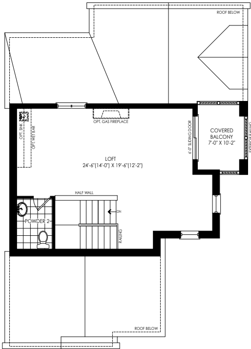
LOFT PLAN ELEV. 'E'
