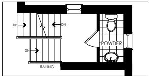
PARTIAL GROUND FLOOR PLAN FOR OPT. FINISHED BASEMENT LANDING ELEV. 'E'
