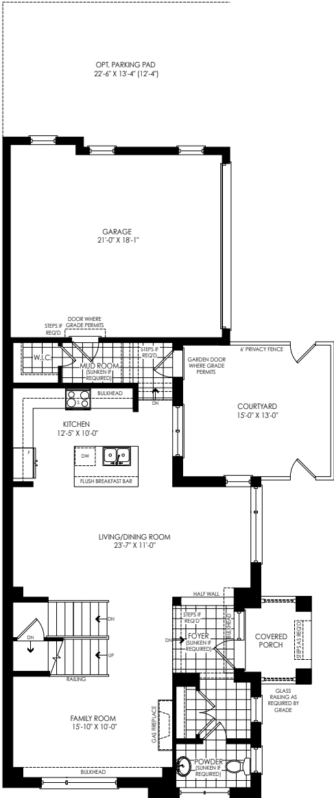
GROUND FLOOR PLAN ELEV. 'A'
