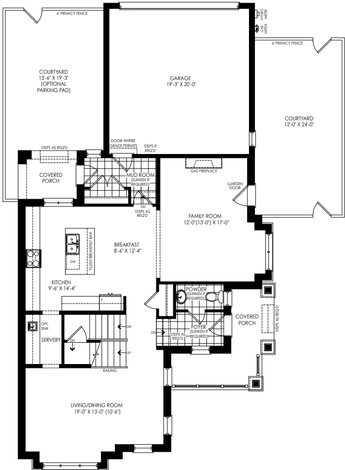
GROUND FLOOR PLAN ELEV. 'B'
