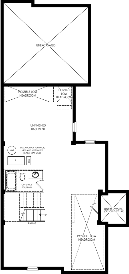
BASEMENT PLAN ELEV. 'A'
