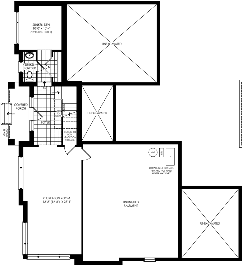
GROUND FLOOR PLAN ELEV. 'A'
