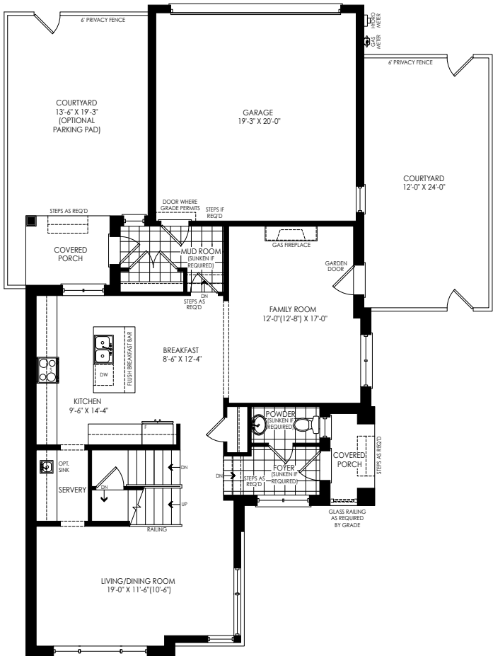
GROUND FLOOR PLAN ELEV. 'A'
