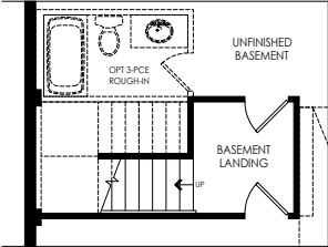
PARTIAL OPT. BASEMENT PLAN W/ FINISHED LANDING ELEV. 'B', 'E' & 'A'
