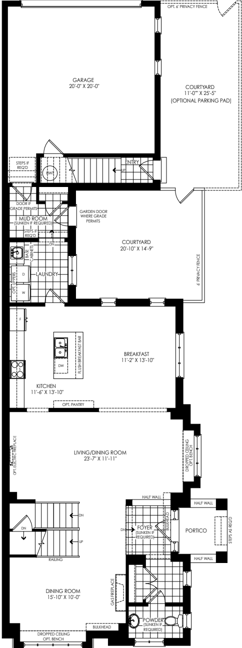
GROUND FLOOR PLAN ELEV. 'E'
