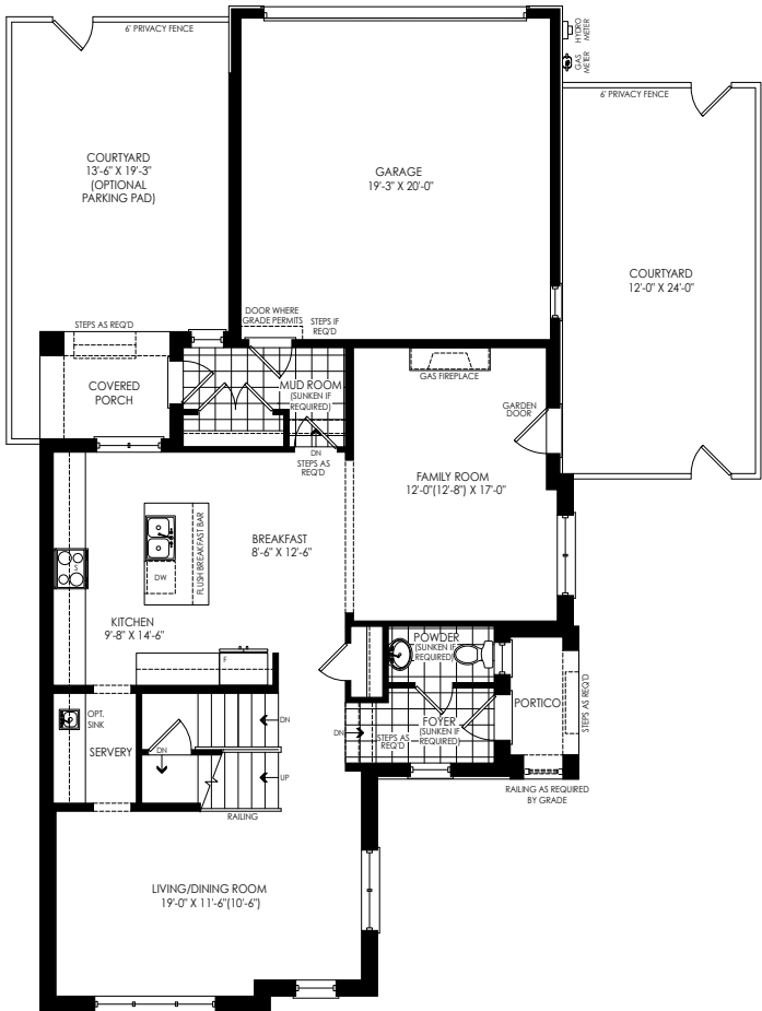
GROUND FLOOR PLAN ELEV. 'D'
