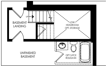
PARTIAL OPT. BASEMENT PLAN W/ FINISHED LANDING ELEV. 'E'
