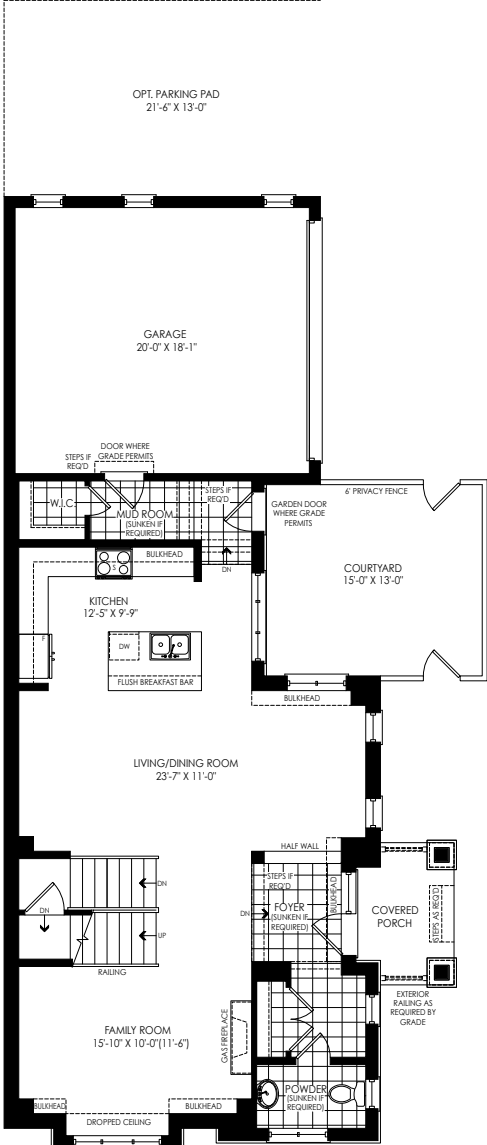
GROUND FLOOR PLAN ELEV. 'B'
