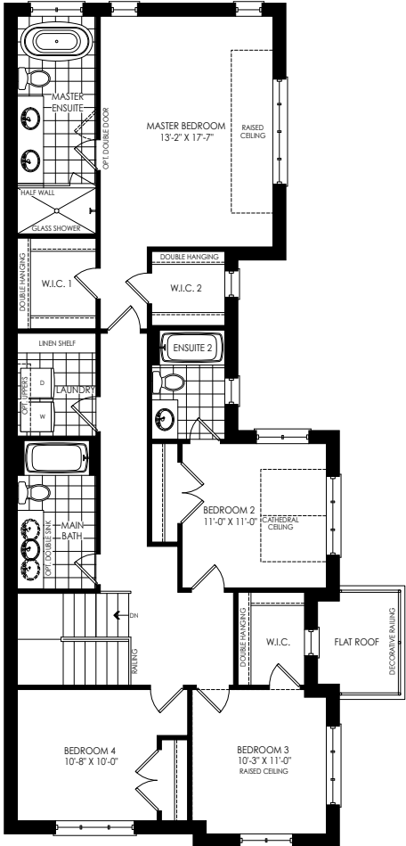
SECOND FLOOR PLAN ELEV. 'E'
