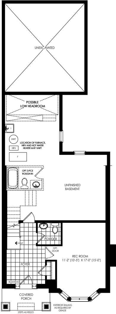
GROUND FLOOR PLAN ELEV. 'B'
